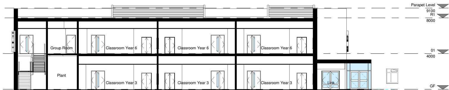
NEW BUILD - SECTION AA
